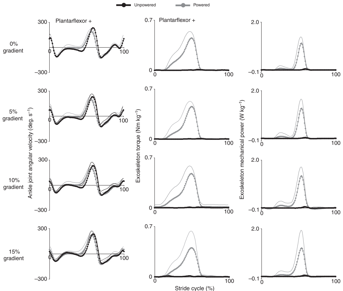
Fig. 3. Ankle exoskeleton mechanics. The thick lines are mean ankle joint angular velocity (left column), exoskeleton torque (middle column) and exoskeleton mechanical power (right column) over the stride from heel strike (0%) to heel strike (100%) of nine subjects. Data are average of left and right legs. Each row is walking data at 1.25 \text{ m s}^{-1} on a single surface gradient (0%-level at top to 15%-uphill at bottom). In each subplot, bold lines are for unpowered (black circles), and powered (gray circles) walking, and thin lines are +1 s.d. Stance is \sim 0\text{--}60\% of the stride, swing 60\text{--}100\% . Ankle joint angular velocity ( \text{deg. s}^{-1} ) is positive for ankle plantarflexion. Exoskeleton torque that acts to plantarflex the ankle is positive. Torque is the product of artificial muscle load and moment arm length and is normalized by subject mass ( \text{Nm kg}^{-1} ). Exoskeleton mechanical power is the product of exoskeleton torque and ankle joint angular velocity and is normalized by subject mass ( \text{W kg}^{-1} ). Positive exoskeleton power indicates transfer of energy from exoskeletons to the user's biological ankle muscle-tendon system.
