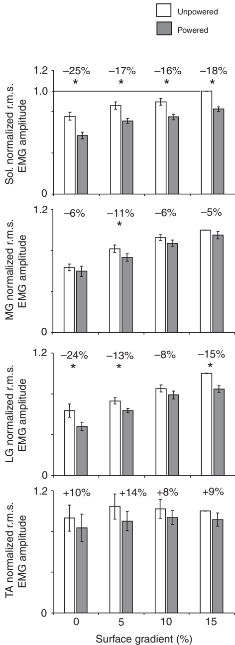
Fig. 5. Ankle muscle root mean square electromyography (EMG) for soleus (Sol.; top), medial gastrocnemius (MG), lateral gastrocnemius (LG) and tibialis anterior (TA; bottom). Values are mean stance phase root mean square (r.m.s.) average muscle activation for nine subjects (error bars are \pm 1 s.e.m.). Surface gradients increase from left (0%-level) to right (15%-uphill) with unpowered walking (minutes 4–6) in white and powered walking (minutes 4–6) in gray. All r.m.s. values (unitless) are normalized to the unpowered 15% grade condition. Values above bars indicate percentage difference in powered versus unpowered condition. Asterisks indicate a statistically significant difference between powered and unpowered walking (ANOVA, P < 0.05 ).
