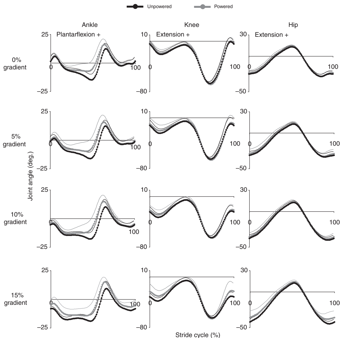
Fig. 2. Joint kinematics. Thick lines are the mean ankle (left column), knee (middle column) and hip (right column) joint angles over the stride from heel strike (0%) to heel strike (100%) of nine subjects. Data are averages of left and right legs. Each row is walking data at 1.25 \text{ m s}^{-1} on a single surface gradient (0%-level at top to 15%-uphill at bottom). In each subplot, curves are for unpowered (black circles), and powered (gray circles) walking and thin lines are +1 s.d. Stance is \sim 0 –60% of the stride, swing 60–100%. For all joints 0 deg. is upright standing posture. Ankle joint plantarflexion, knee joint extension and hip joint extension are all positive.
