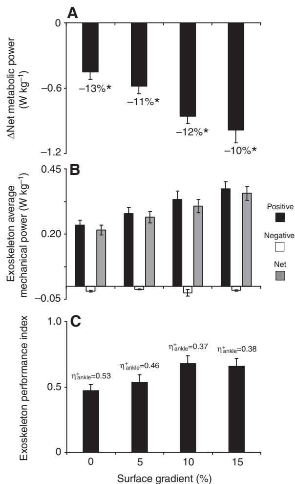
Fig. 4. Exoskeleton performance. Bar graphs show the mean (A) change in net metabolic power (powered–unpowered; \text{W kg}^{-1} ) as a result of powered assistance from bilateral ankle exoskeletons, (B) exoskeleton average positive (black), negative (white) and net (dark gray) mechanical power ( \text{W kg}^{-1} ) over a stride for powered walking and (C) exoskeleton performance index (unitless) of the nine subjects. Performance index indicates the fraction of ankle muscle–tendon positive work performed by plantar flexor muscle shortening rather than Achilles’ tendon recoil (i.e. muscle work fraction). Numbers above bars are equivalent ankle muscle–tendon ‘apparent efficiency’ values (see Materials and methods for details). For all panels, surface inclines increase from left (0%-level) to right (15%-uphill). Error bars are \pm 1 s.e.m. Asterisks (in A) indicate statistical significance for comparison of powered versus unpowered net metabolic power ( P < 0.05 ).
